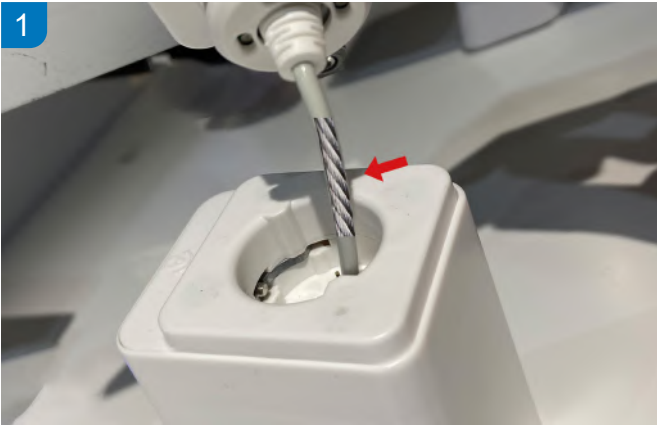
1 Combination of two-core steel wire rope and physical cable puller
