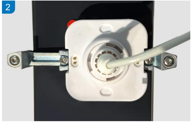
2 The width of the metal clip can be adjusted to suit different commodities
